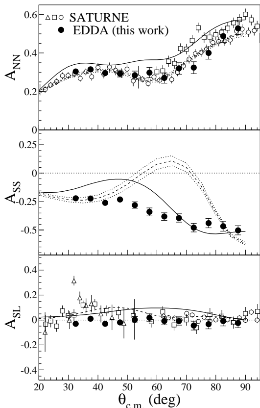
Fig. 1. Angular distributions of the spin correlation parameter A_{NN} , A_{SS} , and A_{SL} at p = 2572 MeV/c ( T_p = 1.8 GeV) in comparison to phase shift predictions of SAID (SM00, solid) [7] and the Saclay-Geneva (dashed line) analysis [8] and data from SATURNE [24]. The EDDA data are preliminary.
